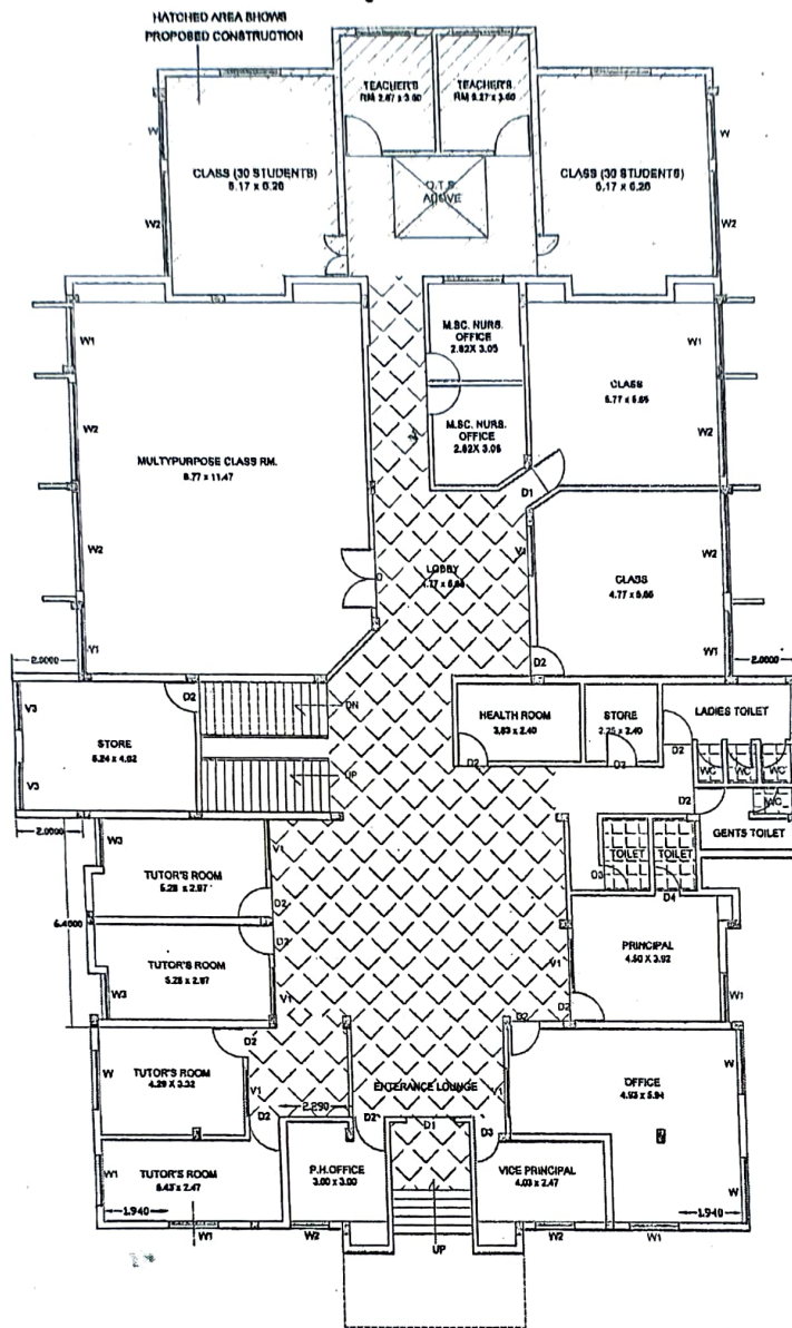
REVISED GROUND FLOOR PLAN
