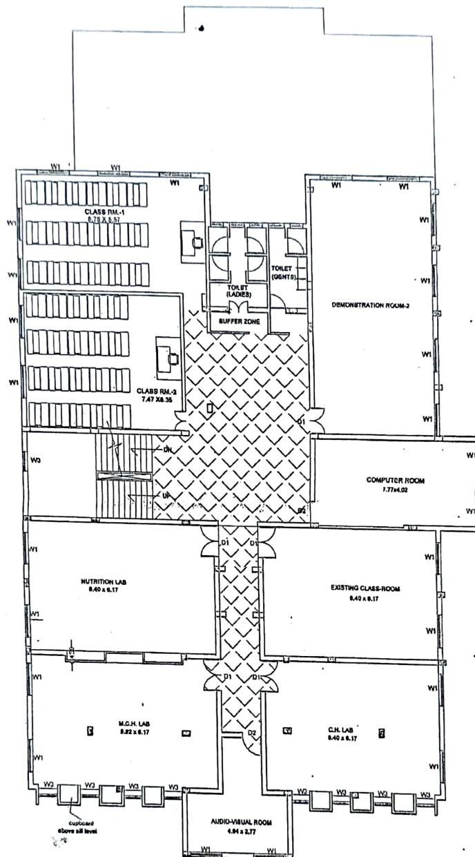
REVISED SECOND FLOOR PLAN
